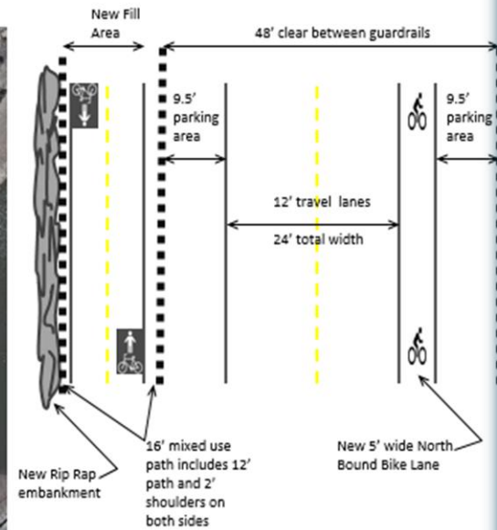
Stanfield Cutoff Connectivity Project Proposed Plan view:
